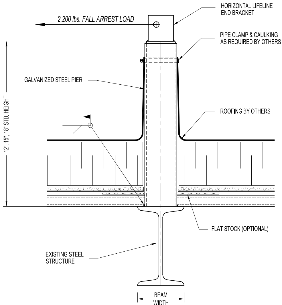
HLL-75E-0000: WELD TO STRUCTURE HLL END ANCHOR
