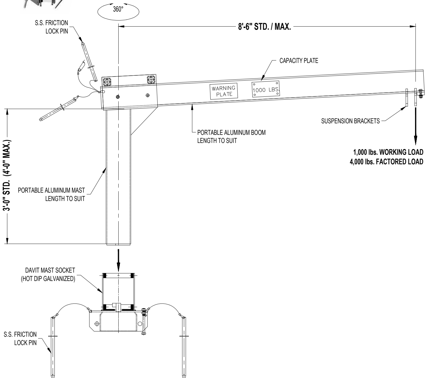
DAVIT ARM ASSEMBLY - A200 (FRONT LOADED) c/w SOCKET
