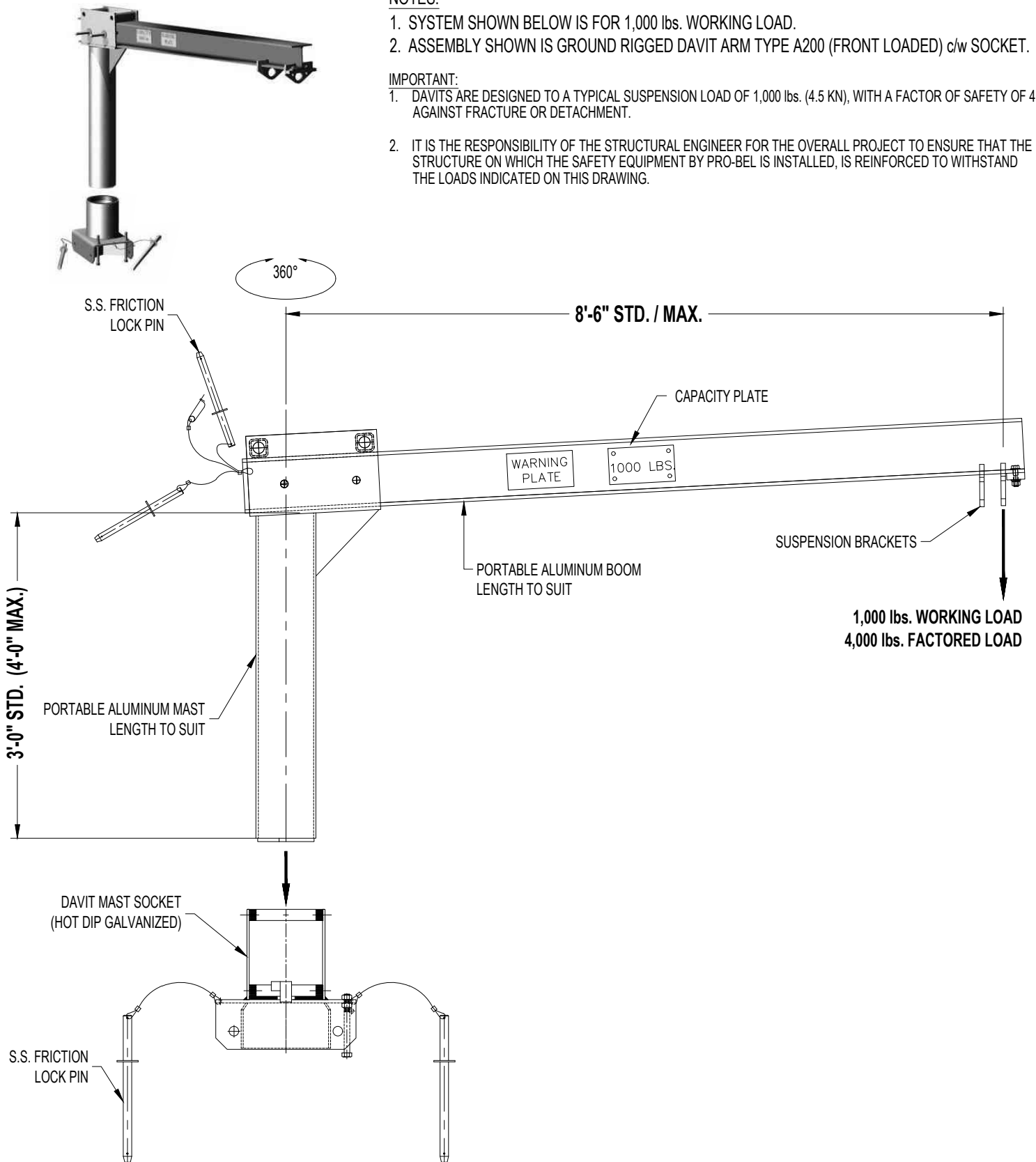
DAVIT ARM ASSEMBLY - A200 (FRONT LOADED) c/w SOCKET
