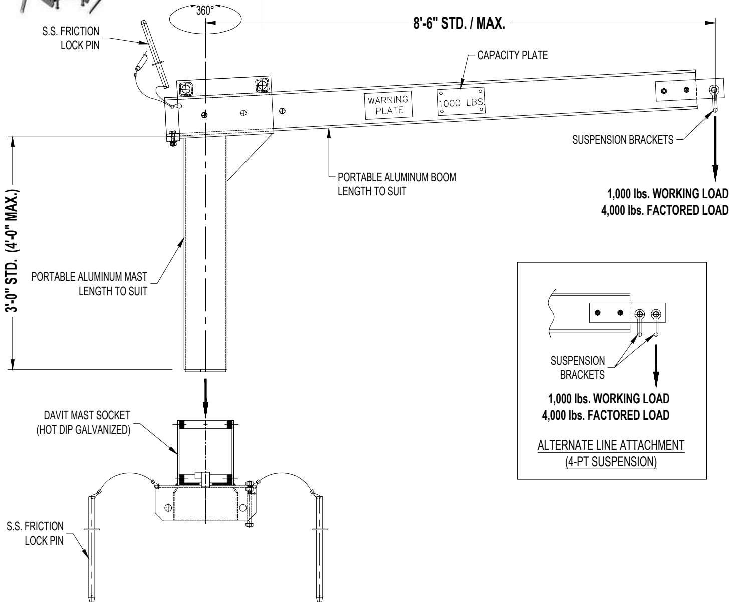
DAVIT ARM ASSEMBLY - A200 (REAR LOADED) c/w SOCKET
