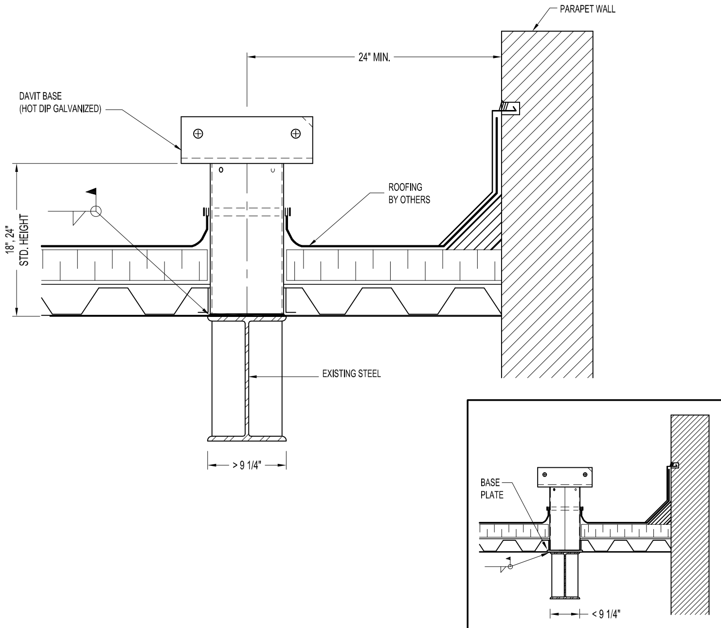
DB2-2300A: 200 SERIES DAVIT BASE ASSEMBLY - (WELD TO STEEL) - WITHOUT U-BAR
