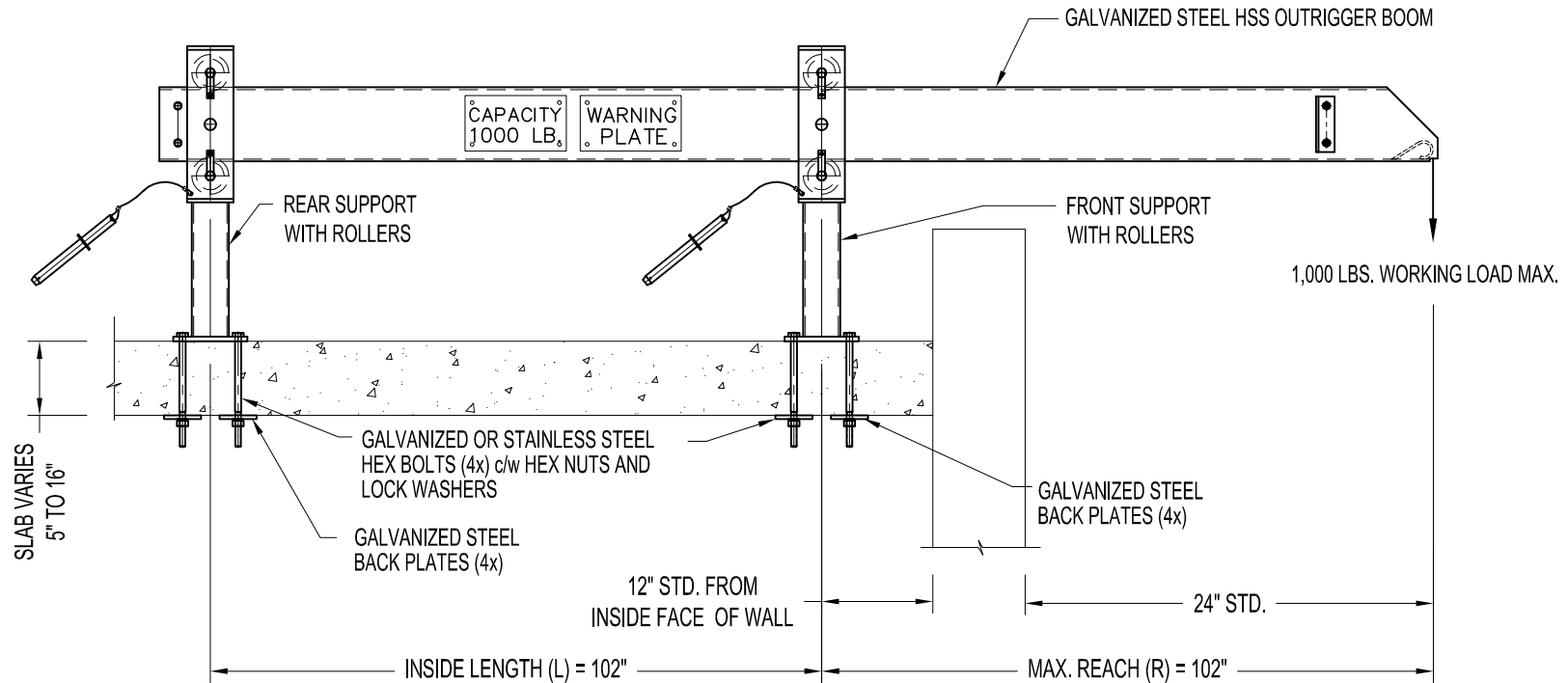
A-OR-1140-102: FIXED OUTRIGGER ASSEMBLY (UP TO 8'-6 REACH) - BOLT THROUGH
