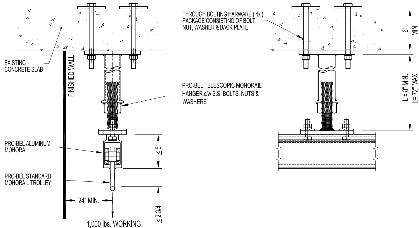
MNH310-7200: PRO-BEL MONORAIL HANGER BRACKET ASSEMBLY TYPE 3 - (THROUGH BOLTED)
