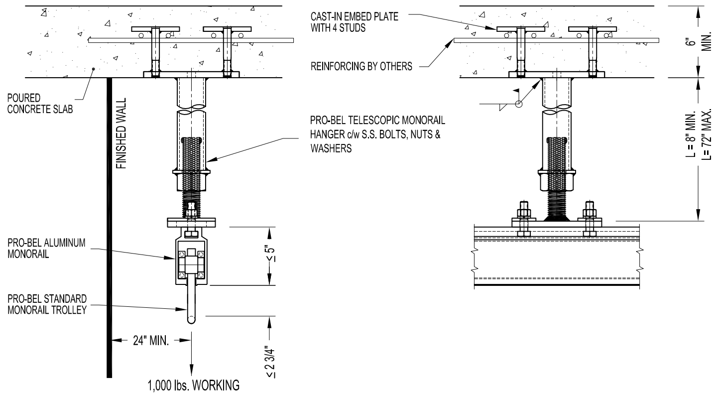
MNH380-7200: PRO-BEL MONORAIL HANGER BRACKET ASSEMBLY TYPE 3 - (WELD TO CAST-IN EMBED)
